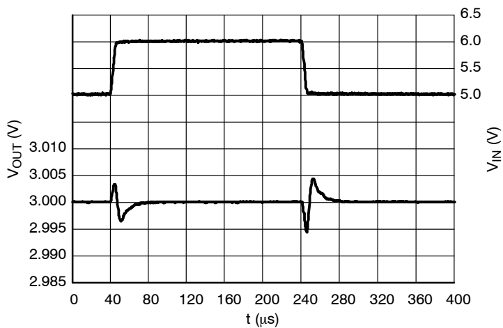
Figure 52. Line Transients, 3.0 V Version, t_R = t_F = 5 \mu s, I_{OUT} = 30 mA, ECO = H
