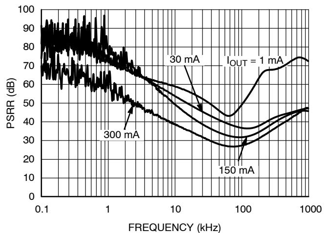
Figure 44. PSRR, 5.0 V Version, V_{IN} = 8.0 V, ECO = H
