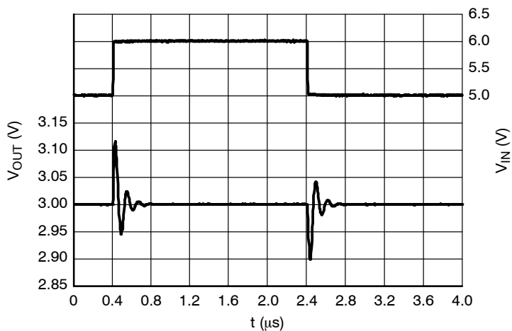
Figure 51. Line Transients, 3.0 V Version, t_R = t_F = 5 \mu s, I_{OUT} = 30 mA, ECO = L
