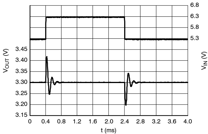
Figure 53. Line Transients, 3.3 V Version, t_R = t_F = 5 \mu s, I_{OUT} = 30 mA, ECO = L
