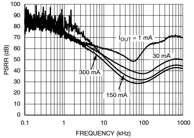
Figure 40. PSRR, 3.0 V Version, V_{IN} = 6.0 V, ECO = H
